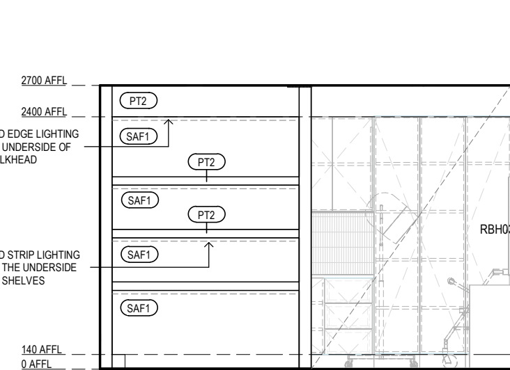
VILLAGE HEALTH & WELLNESS - SALON ELEVATION 3 Scale 1: 50
