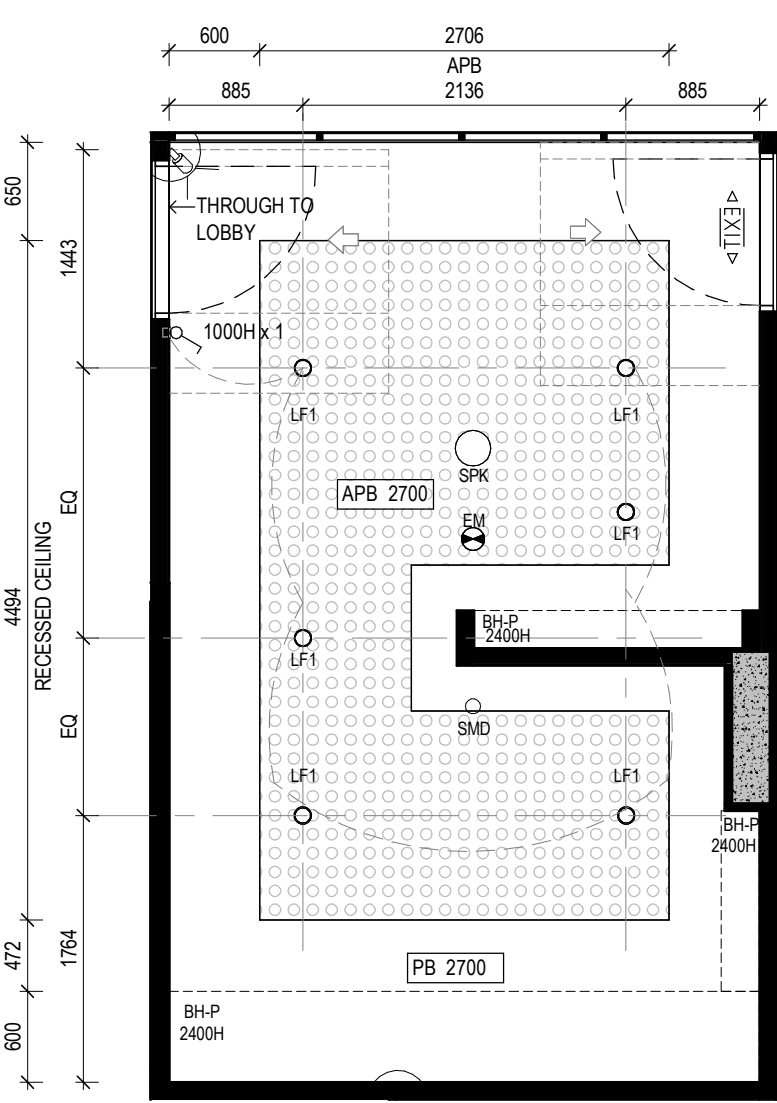
2 RCP - VILLAGE HEALTH & WELLNESS - SALON Scale 1: 50
