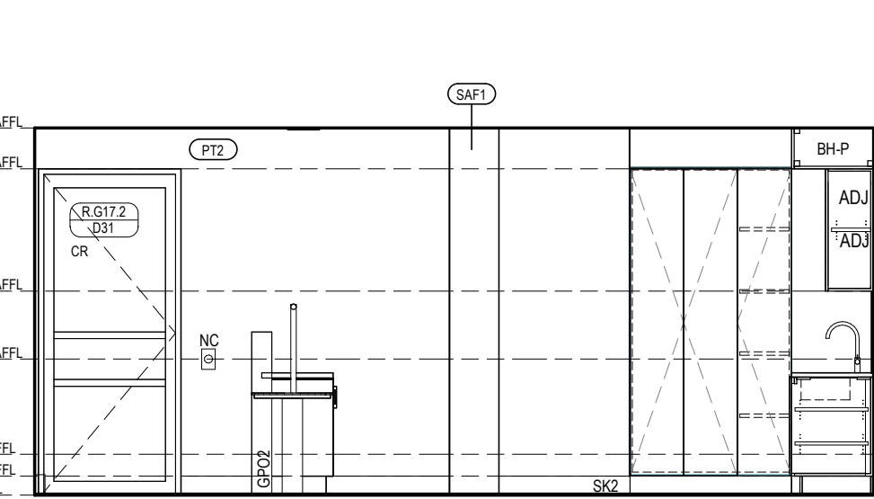
VILLAGE HEALTH & WELLNESS - SALON ELEVATION 1 Scale 1: 50
