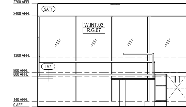
VILLAGE HEALTH & WELLNESS - SALON ELEVATION 4 Scale 1: 50
