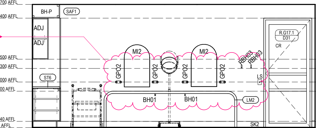
VILLAGE HEALTH & WELLNESS - SALON ELEVATION 2 Scale 1: 50
