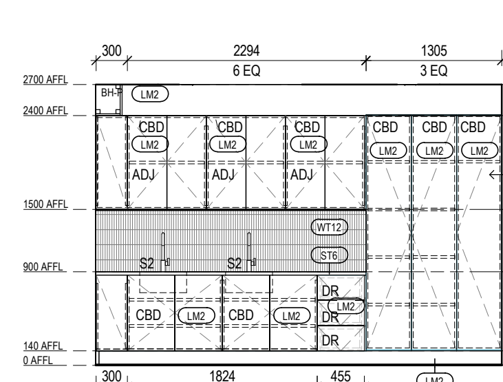
VILLAGE HEALTH & WELLNESS - SALON ELEVATION 2A Scale 1: 50
