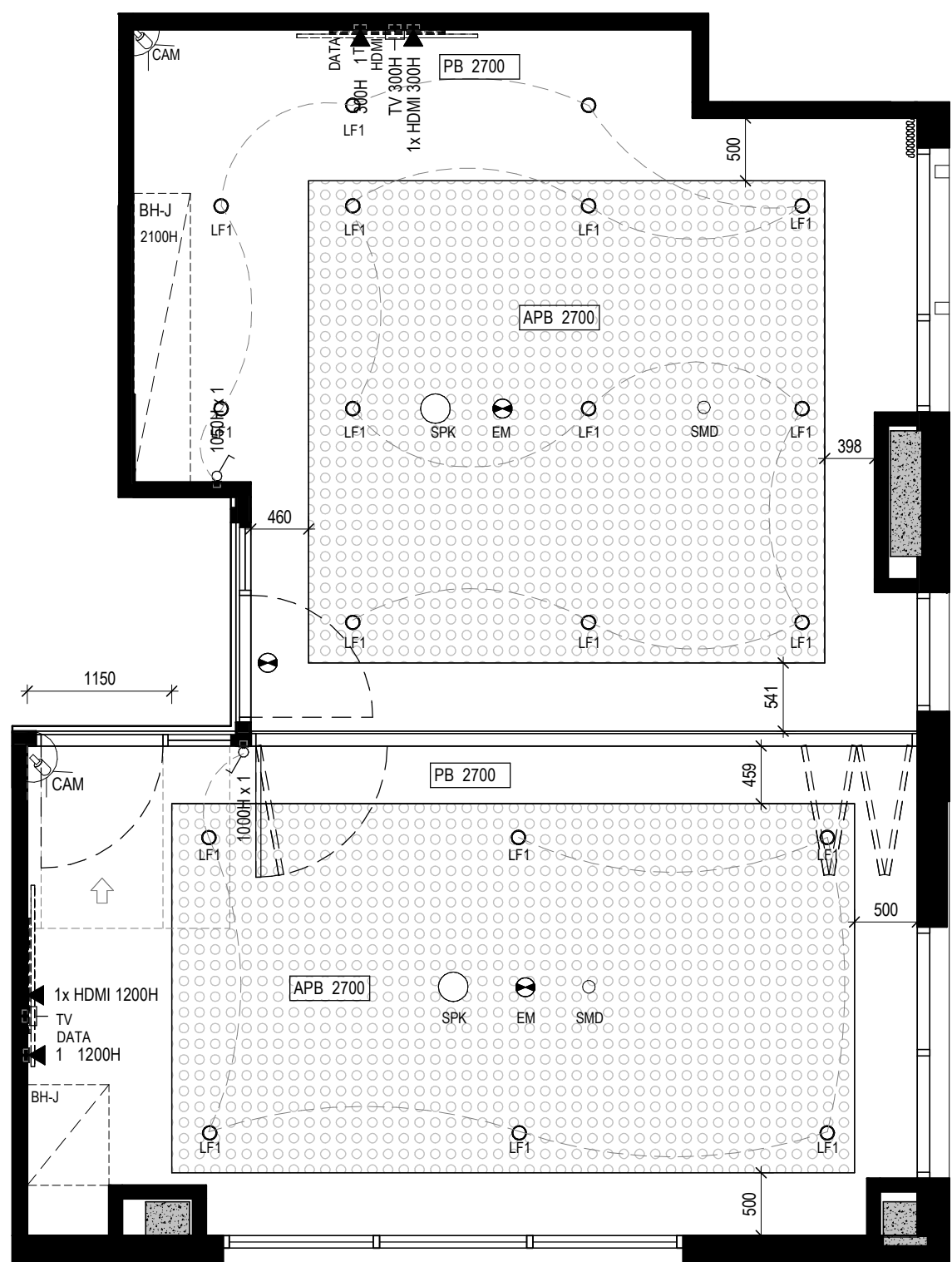
6 RCP - VILLAGE HEALTH & WELLNESS - GYM Scale 1: 50
