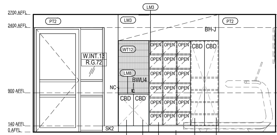
VILLAGE HEALTH & WELLNESS - GYM ELEVATION 4 Scale 1: 50
