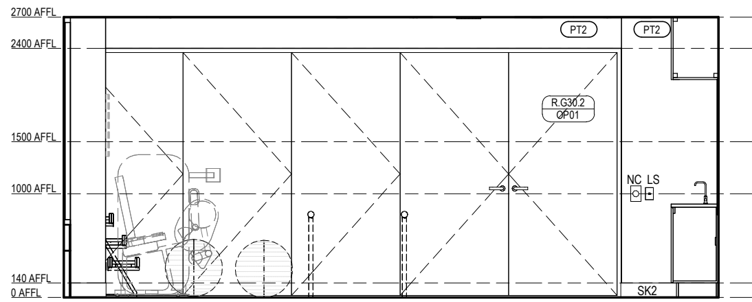
VILLAGE HEALTH & WELLNESS - GYM ELEVATION 3 Scale 1: 50
