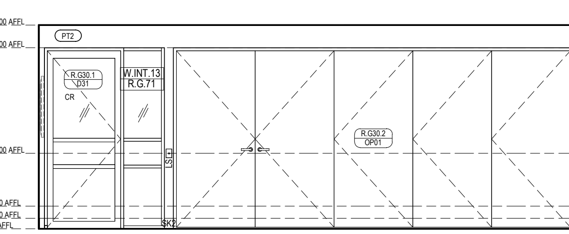
VILLAGE HEALTH & WELLNESS - FLEX ELEVATION 1 Scale 1: 50
