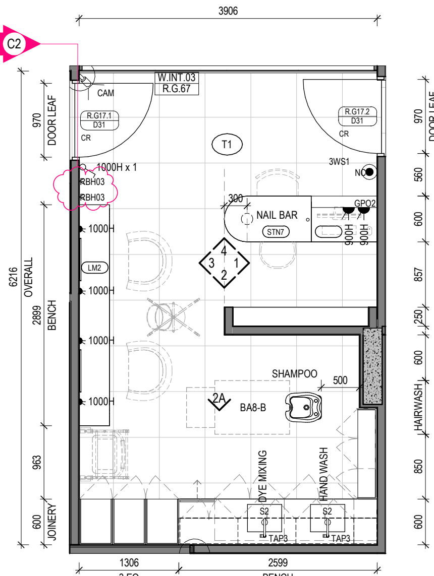
1 VILLAGE HEALTH & WELLNESS - SALON Scale 1: 50
