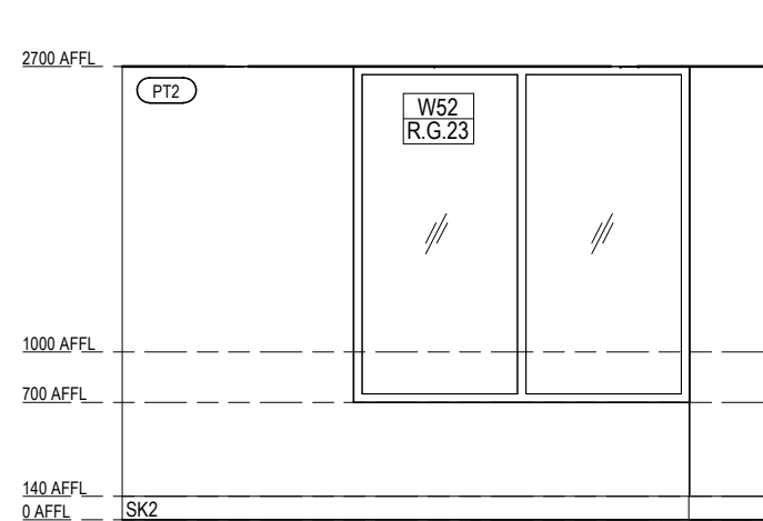
VILLAGE HEALTH & WELLNESS - FLEX ELEVATION 2 Scale 1: 50
