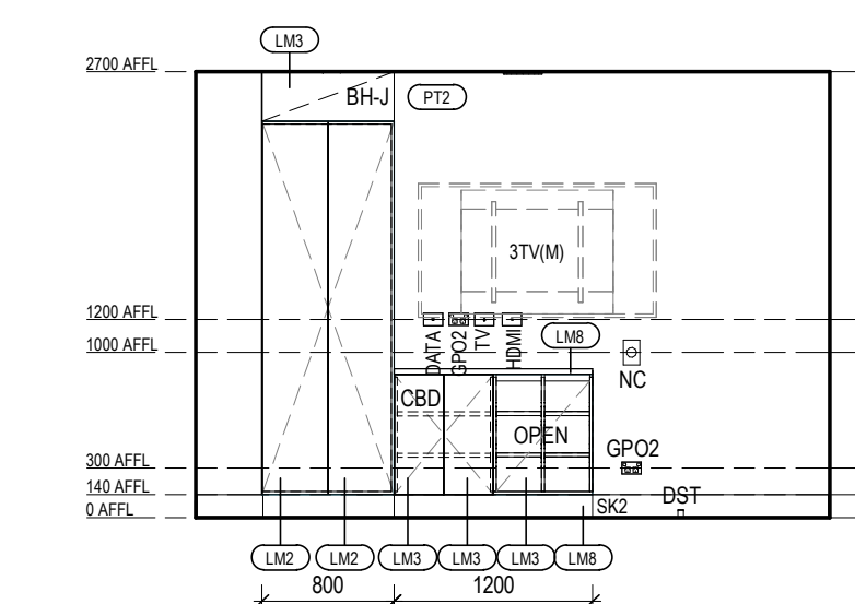
VILLAGE HEALTH & WELLNESS - FLEX ELEVATION 4 Scale 1: 50
